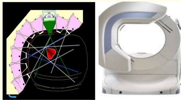
Figure 4: Cadmium-zinc-telluride semiconductor detector. In digital semiconductor gamma cameras with direct gamma radiation conversion, one aperture on the collimator corresponds to one semiconductor detection unit and simultaneously to one resulting image point (pixel).
