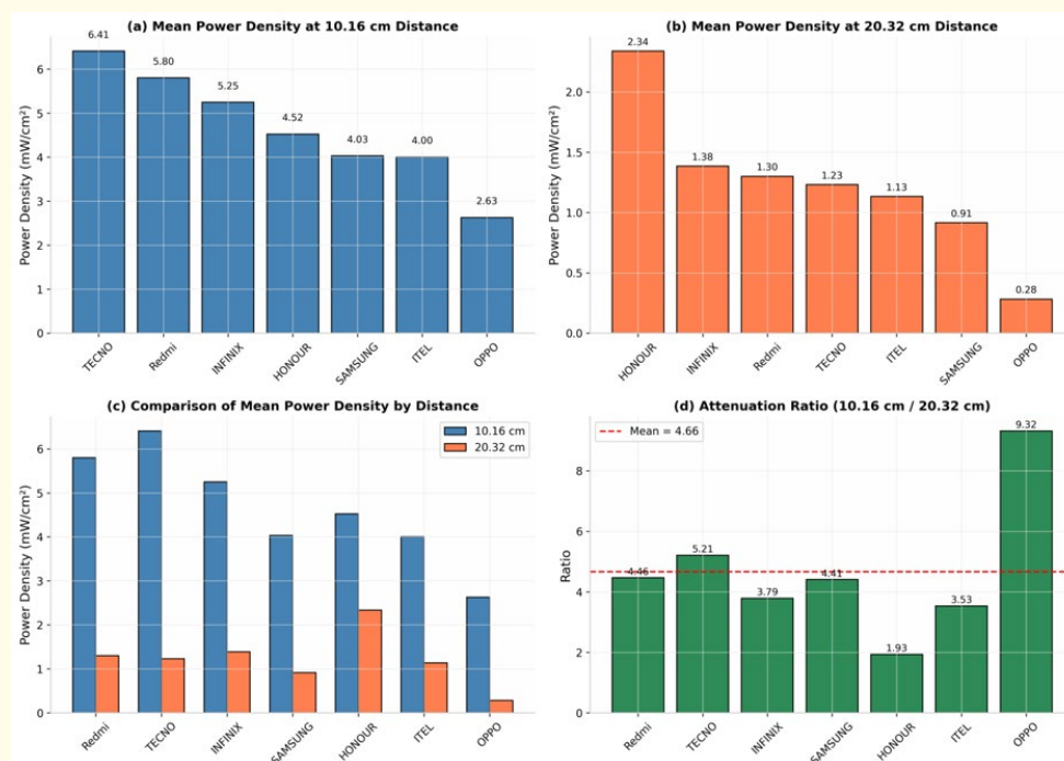
Figure 1: Comparative analysis of RF power density emissions by mobile phone brand: (a) mean power density at 10.16 cm distance; (b) mean power density at 20.32 cm distance; (c) side-by-side comparison of mean power density at both distances; (d) computed attenuation ratio (10.16 cm / 20.32 cm) for each brand, with the dashed line indicating the overall mean ratio of 4.66.
