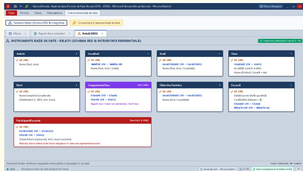
Figure 10: The underlying db schema, including relational integrity.
