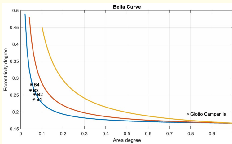
Figure 5: The Bella Curves as shown in figure 2 plotted together with the two considered buildings shown in Table 3.
