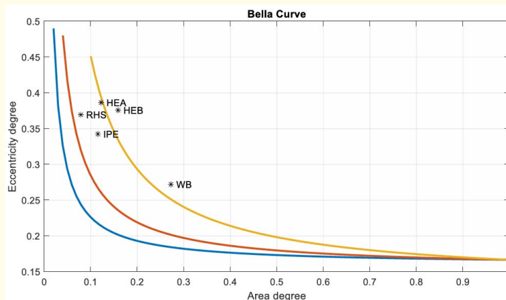
Figure 4: The Bella Curves as shown in figure 2 plotted together with the classical beam sections shown in Table 1.
