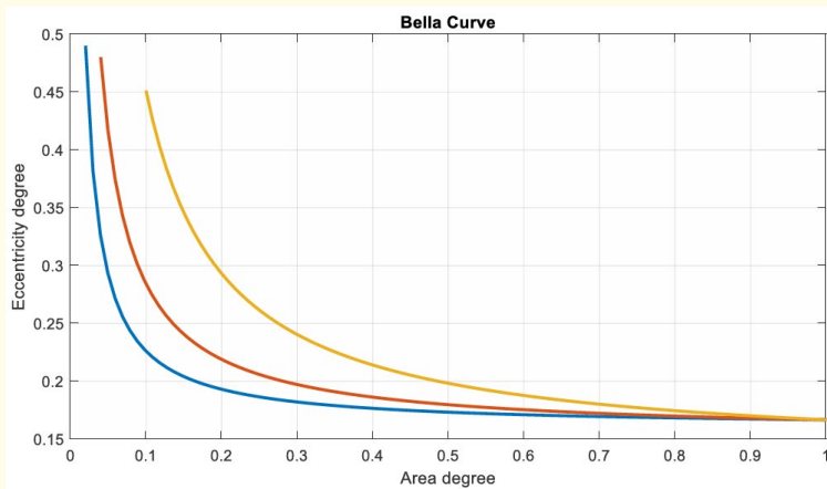
Figure 3: Eccentricity degree defined in Eq. (6) as a function of the area degree A/A_0 . From the bottom the three curves represent cases where the flange thickness is 1, 2 and 5 % of the beam depth.
